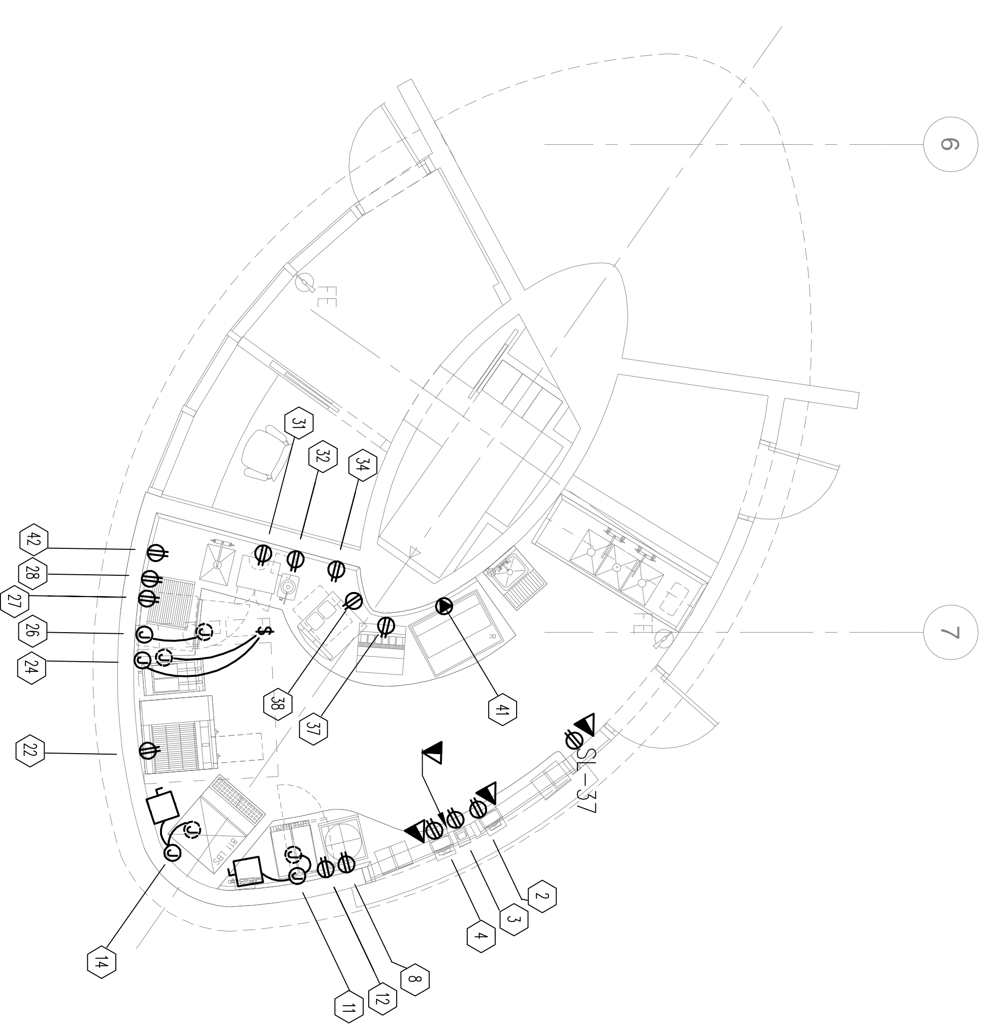
SNACK BAR ENLARGEMENT POWER PLAN Scale: 1/4" = 1'-0"
